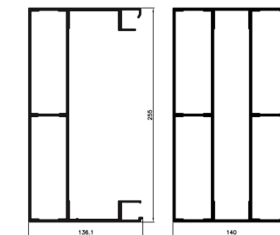
Outer and inner purlins measuring 140×255 mm
